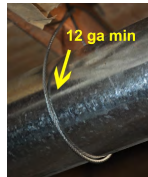
Metal wire should be at least 12 gauge and galvanized
