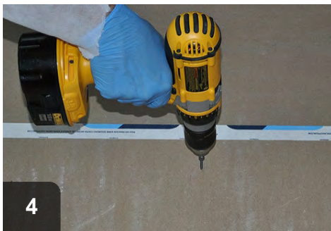
4 Fasten cap with screws to set sealant and create air barrier
