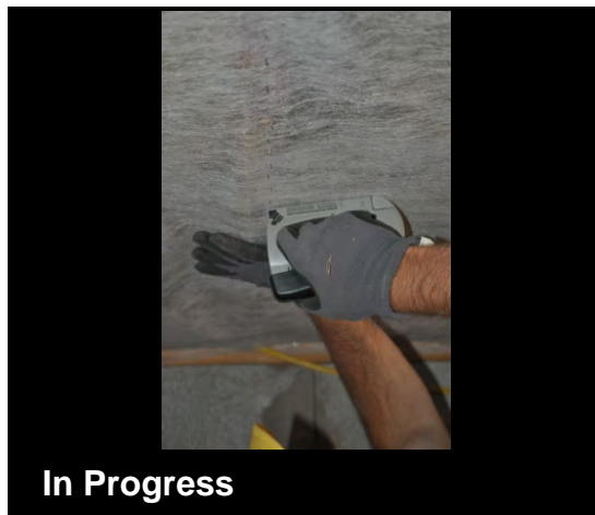
Netting is secured to joists and sills to create cavities for insulation
