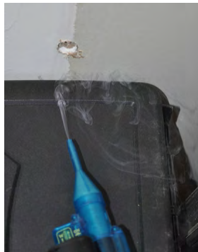
With blower door running, chemical smoke should not draw into test holes
