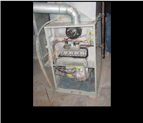
Induced draft furnace
