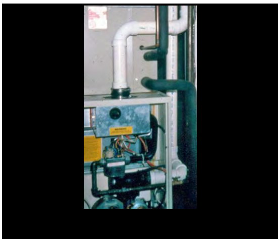
Forced draft appliance with sealed combustion
