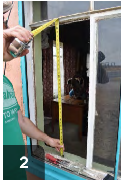
2 With broken glass removed, measure opening for replacement glass
