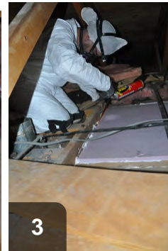
3 Once cap is set, apply sealant to remaining gaps and along all seams
