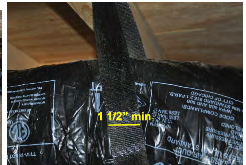
Support straps should be at least 1 1/2 inches wide
