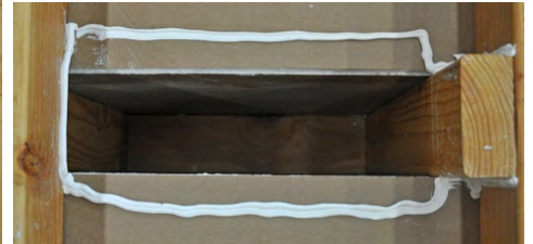
Option 3, Step 1: Apply sealant around opening and on surrounding framing
