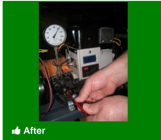
Verify that fuel pressure matches manufacturer's specifications
